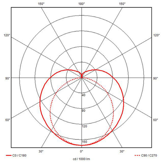
Photometric Diagram
