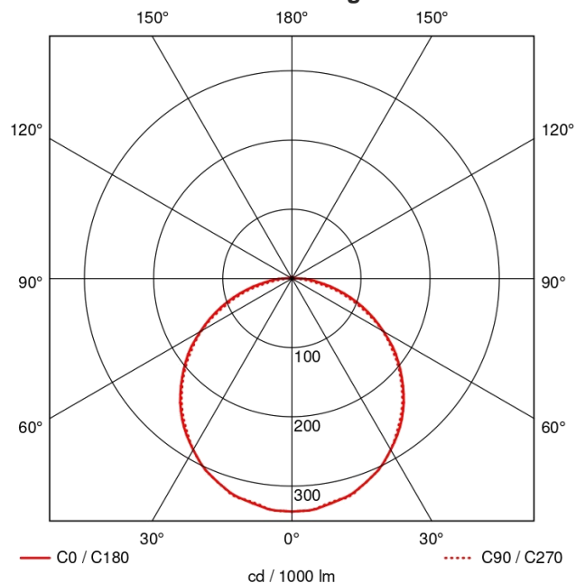
Photometric Diagram
