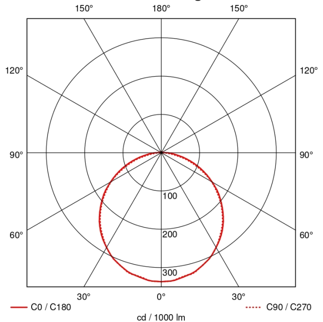
Photometric Diagram
