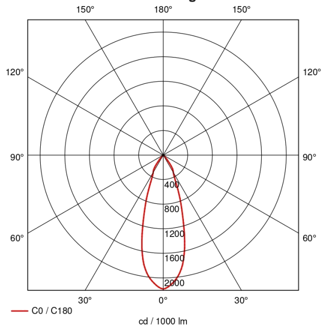
Photometric Diagram
