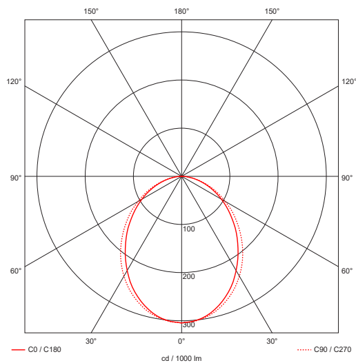
Photometric Diagram
