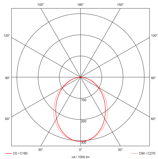
Photometric Diagram
