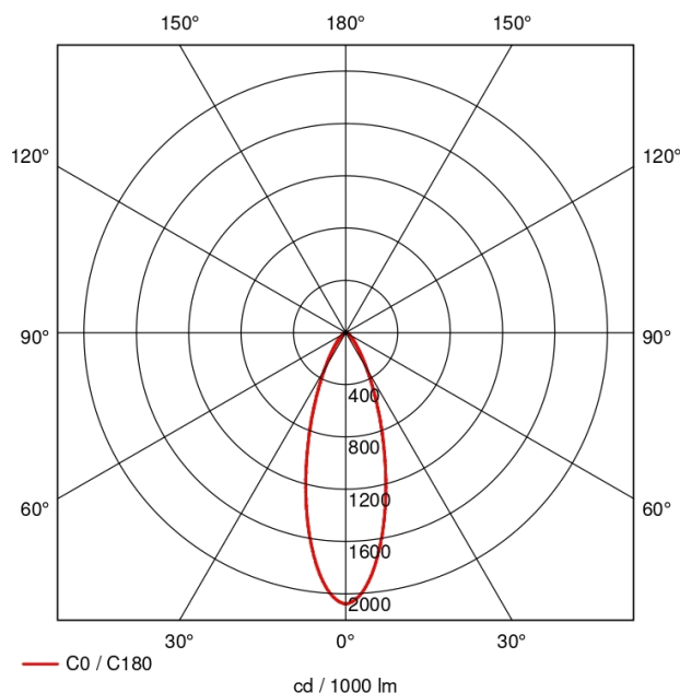
Photometric Diagram
