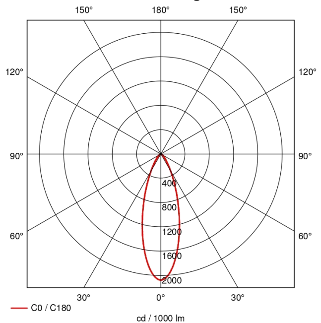
Photometric Diagram
