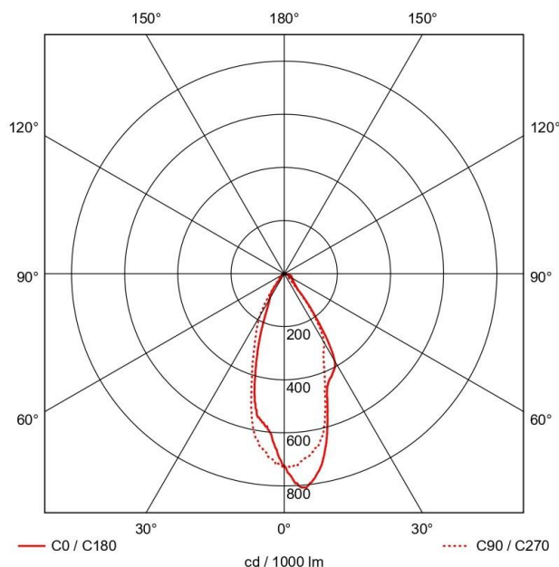
Photometric Diagram
